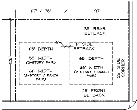
DUPLEX TYPICAL LOT DETAIL SCALE: 1"=50'
