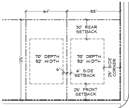
SINGLE FAMILY TYPICAL LOT DETAIL SCALE: 1"=50'
